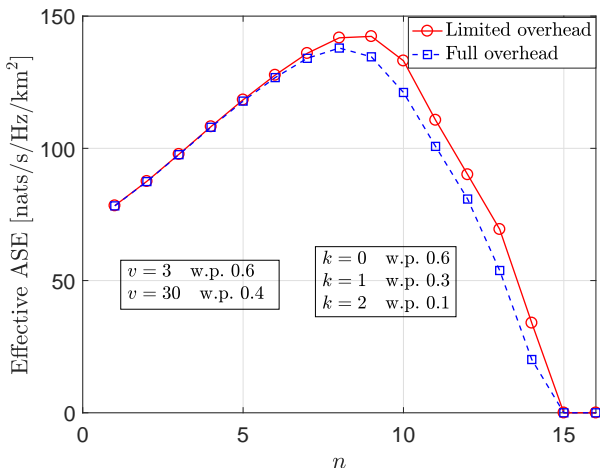
Fig. 10: Overall performance for the mix of MTs. \text{ISD} = 200 m. p_0 = 0.6 , p_1 = 0.3 , and p_2 = 0.1 . q_3 = 0.6 and q_{30} = 0.4 .
