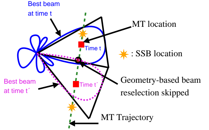
Fig. 2: Mobility-induced beam misalignment. Ideally, the beam reselection should happen at the beam boundary for the MT to stay connected to the main lobe of the best beam. But, since the SSB burst (a beam-formed reference signal) location might not coincide with the location of ideal beam reselection at the beam boundary, the MT at time t' is still connected to the side lobe of the previously selected beam at time t , which results in a beam misalignment.
