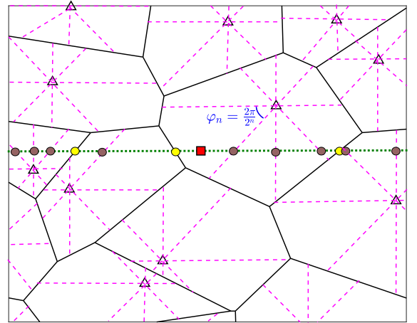
Fig. 1: A snapshot of a Poisson cellular network with directional beamforming to an MT. Here, each BS has 2^3 = 8 beams, i.e., n = 3 . Triangles: Base stations (BSs), Square: MT location, Circles on dashed lines: Geometry-based beam reselection locations, Circles on solid lines: BS handover locations, Solid lines: Cell boundaries, Dashed lines: Beam boundaries, and Dotted line: Trajectory of the MT.
