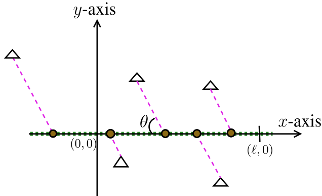
Fig. 11: At most one geometry-based beam reselection for a BS. Triangles: Base station locations, Circles: Beam reselection locations, Dashed lines: Beam boundaries, and Dotted line: MT trajectory along the x -axis.
