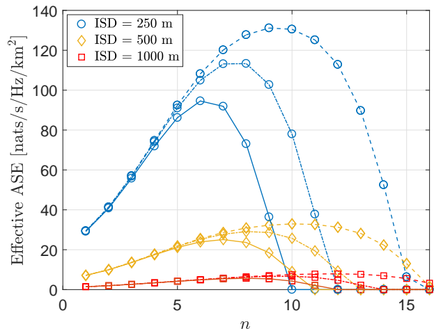
(a) FR1 : Dashed line: v = 3 km/h, Dashed-dotted line: v = 30 km/h, and Solid line: v = 120 km/h.
