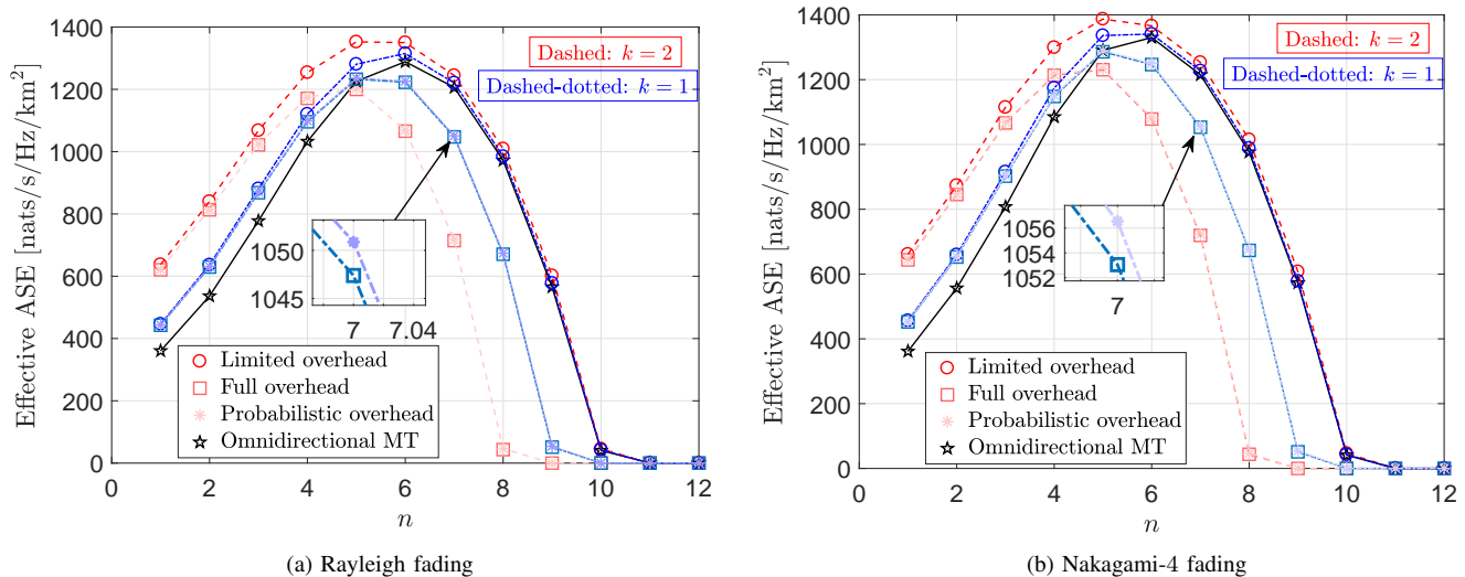
Fig. 6: Effect of the number 2^k beams at the typical MT on the effective ASE. v = 30 km/h and ISD = 75 m.
