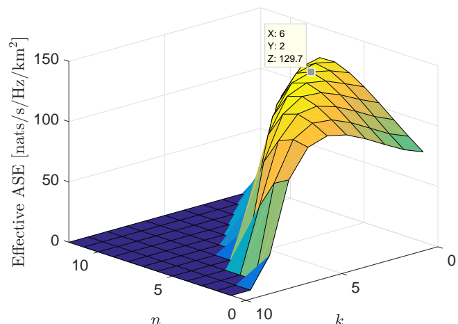
(b) Full overhead case
