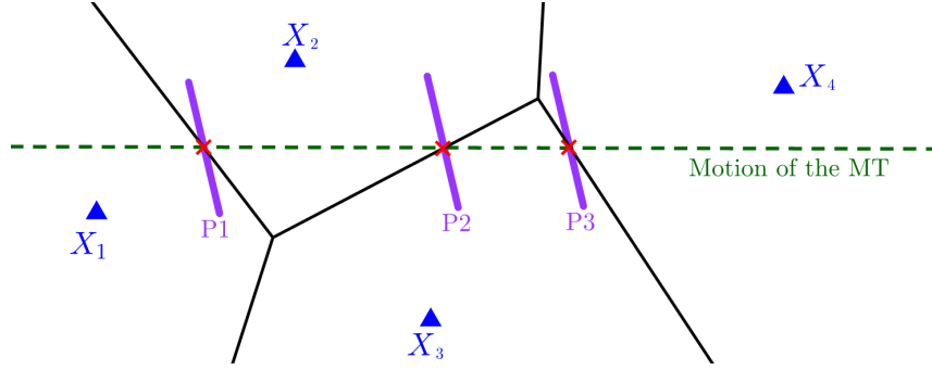
Fig. 3: Probabilistic beam switching with two beams (panels) at the MT. The triangles depict the BSs located according to a PPP. The solid black lines denote cell boundaries. A “cross” denotes the BS handover location of the MT. P1, P2, and P3 denote randomly oriented panels of the MT pertaining to each BS handover location, where each of the two beams covers the left and right halves separated by the panel. For instance, the BSs X_1 and X_2 lie in the coverage of two different beams, i.e., on the opposite side of the panel P1. Thus there will be a beam switch during the handover from X_1 to X_2 . On the contrary, X_2 and X_3 lie in the coverage of the same beam (the left beam). Thus there is no need of a beam switch during the handover from X_2 to X_3 .
